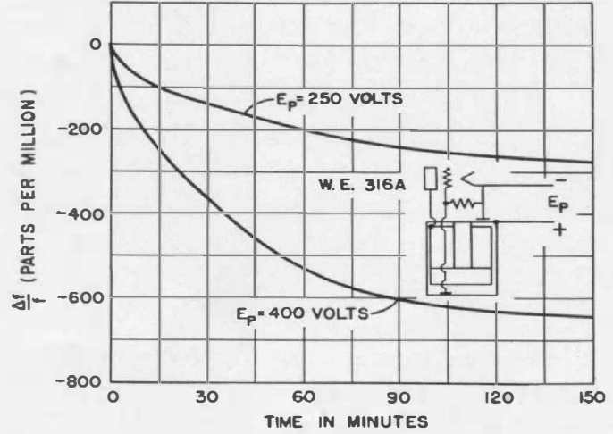
FIGURE 5. Drift in frequency of oscillation during warming-up period at plate voltages of 250 volts and 400 volts
