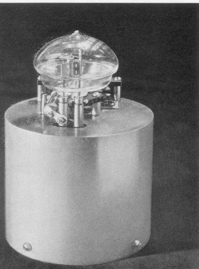
FIGURE 1. The complete oscillator consisting of tank circuit and vacuum tube. The over-all height is 7 inches
