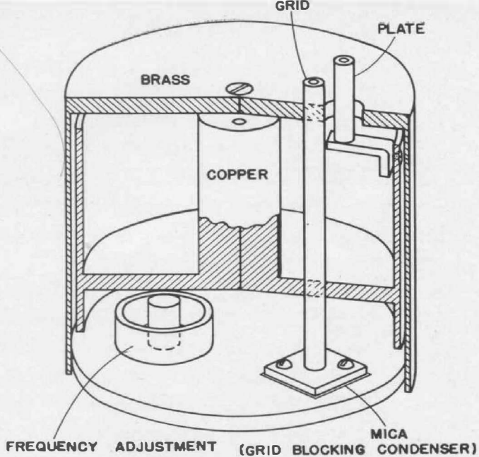
FIGURE 2. Sectional view of the tank circuit showing details of assembly
