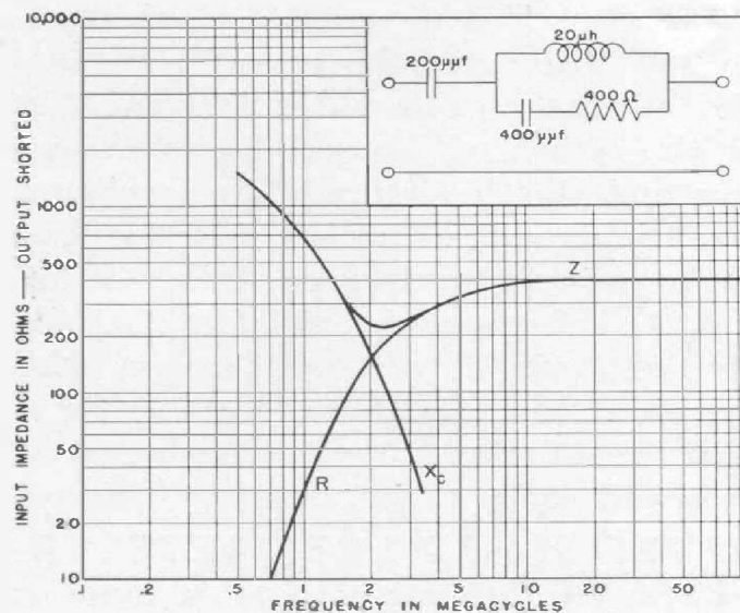
FIGURE 1. Resistance, reactance, and impedance characteristics of the TYPE 418-G Dummy Antenna
