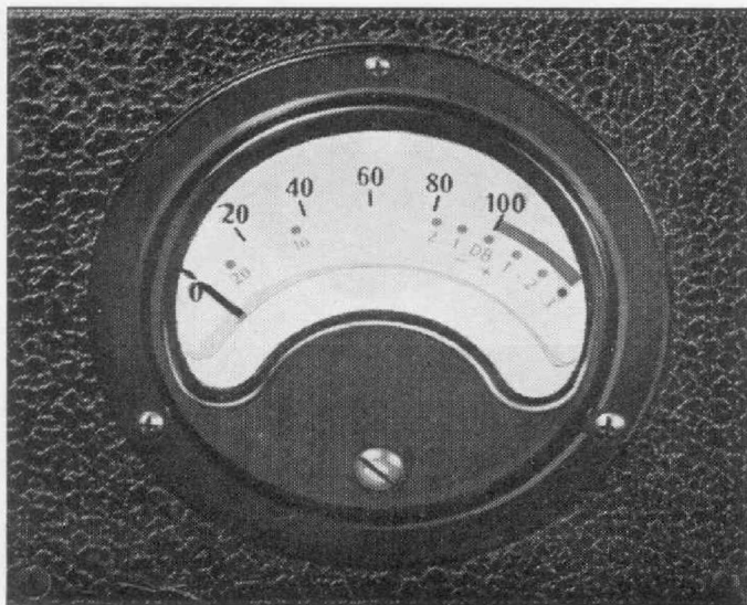
FIGURE 2. Photograph of the indicating meter. The main scale is black on a yellow background. The decibel scale is red. Two lamps behind the panel illuminate the scale
