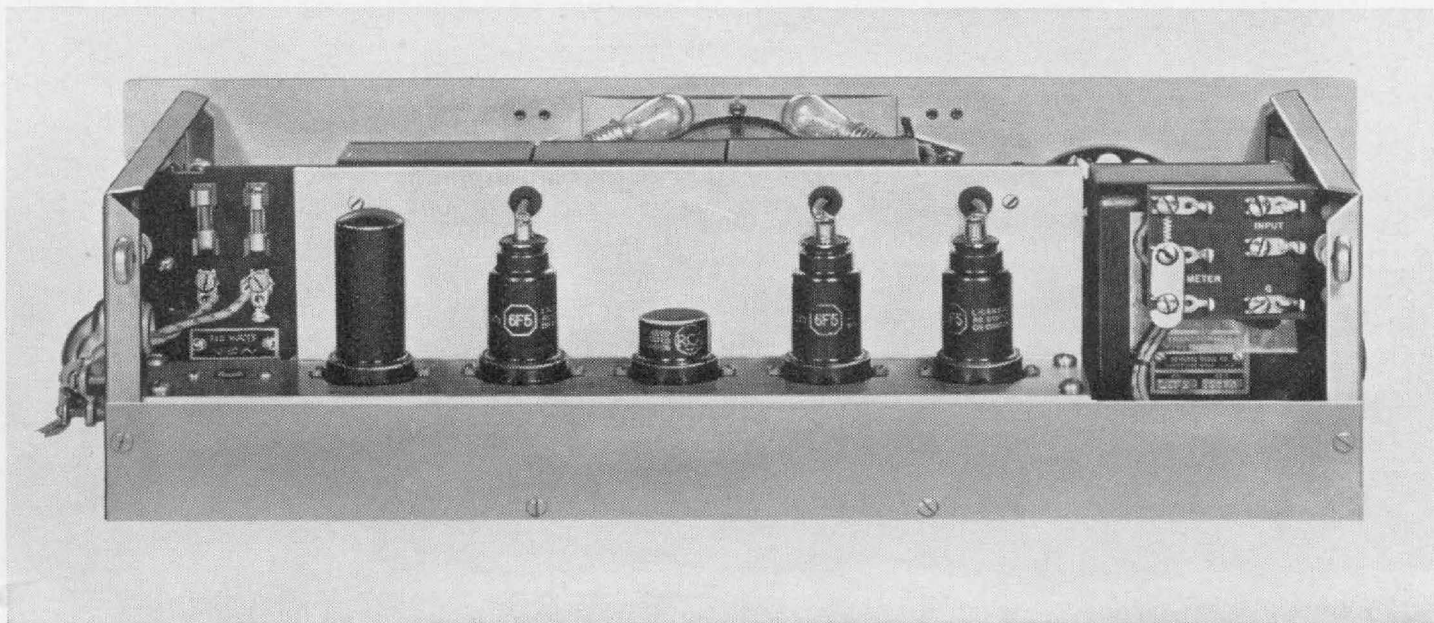
FIGURE 3. Rear view of the power-level indicator with dust cover removed. Note that all tubes are easily accessible from the rear
