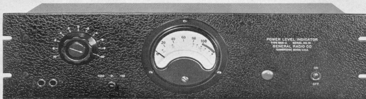
FIGURE 1. Panel view of the TYPE 686-A Power-Level Indicator
