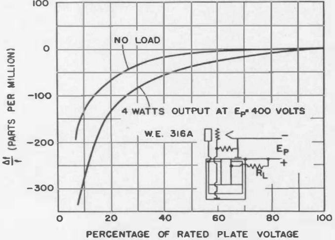
FIGURE 4. Change in frequency produced by a variation in applied plate voltage. The upper curve is taken at no load, the lower with a load of 4 watts
